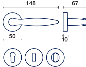
rosette - bocchette 10 mm rosettes - escutcheon
